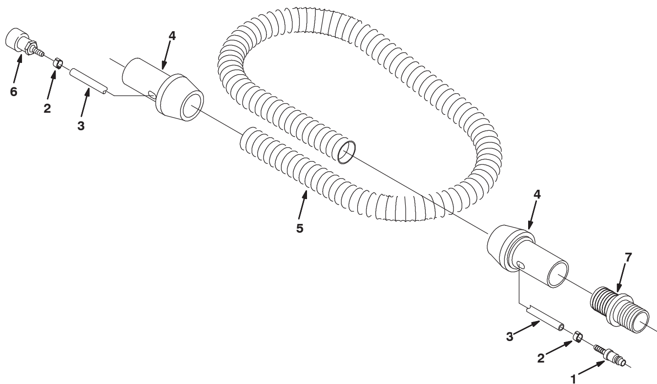
Fig. 46 - Power Wand Hose Assembly
