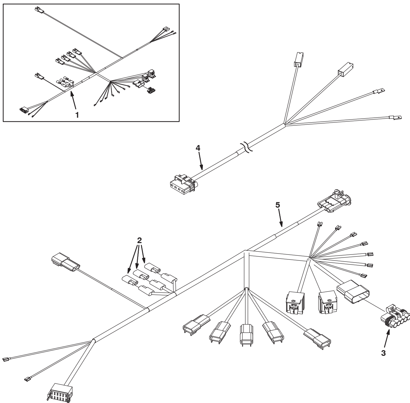
Fig. 65 - FaST Wire Harness Group (0000-1121)
