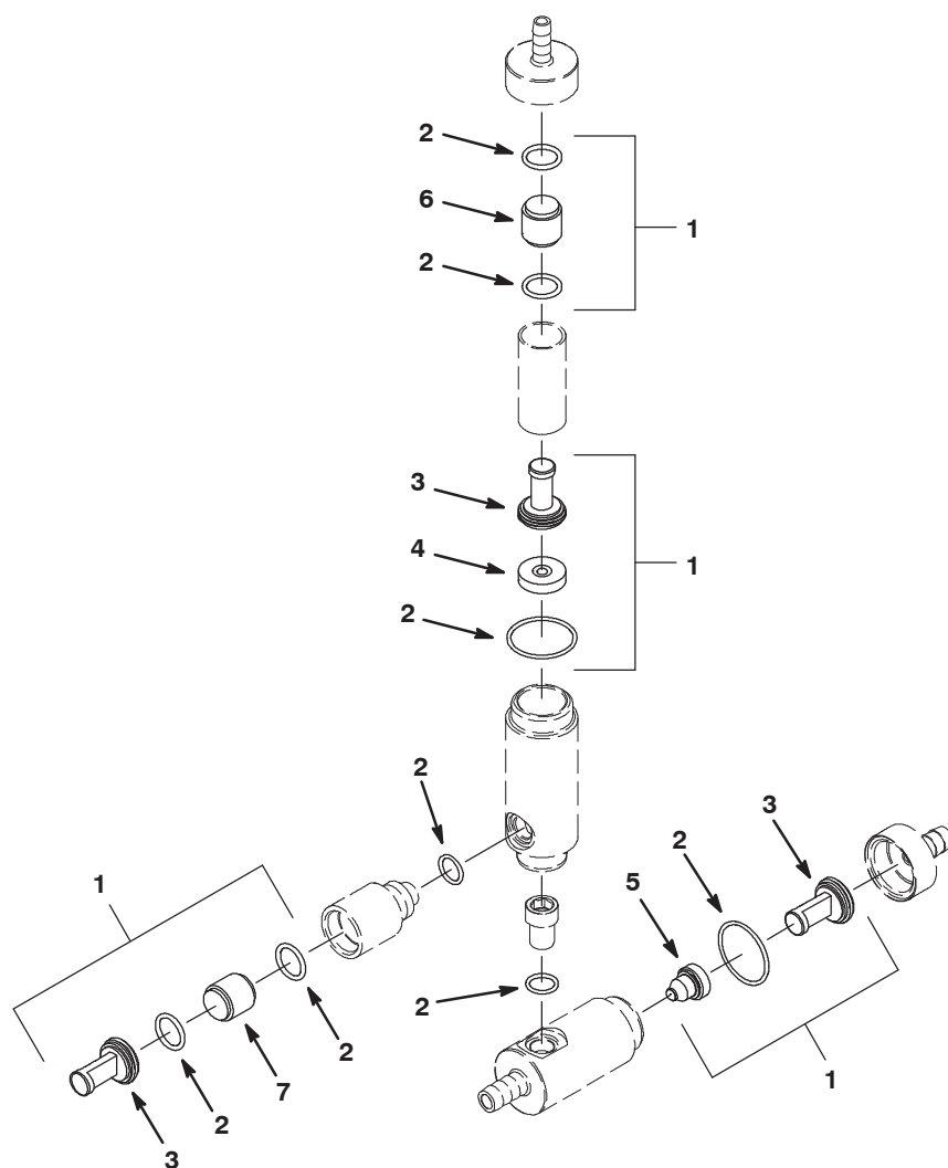
Fig. 20 - FaST Injector Assebmly Breakdown, 1050333
