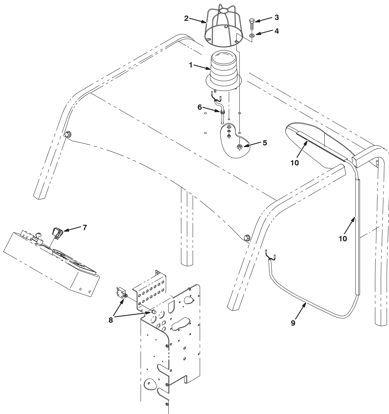
Fig. 2 - Flashing Light Group, Overhead Guard
