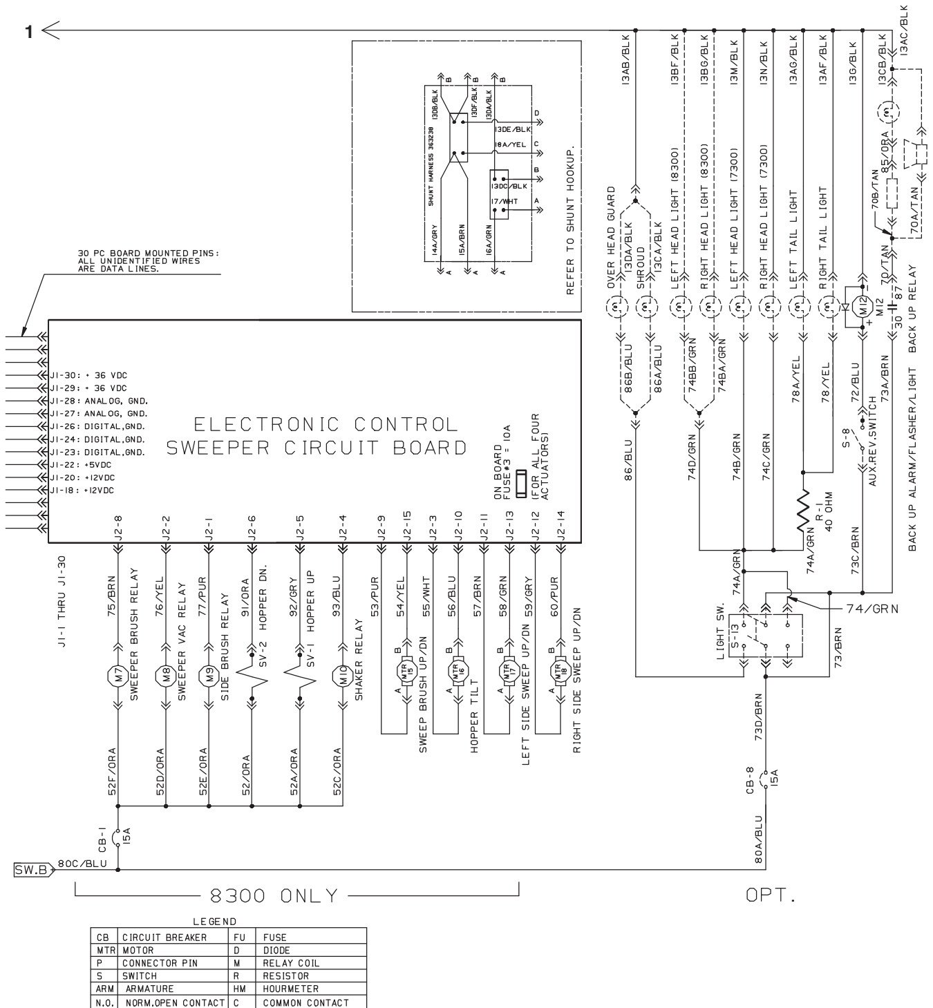
Fig. 63 - Electrical Schematic (1122- )
