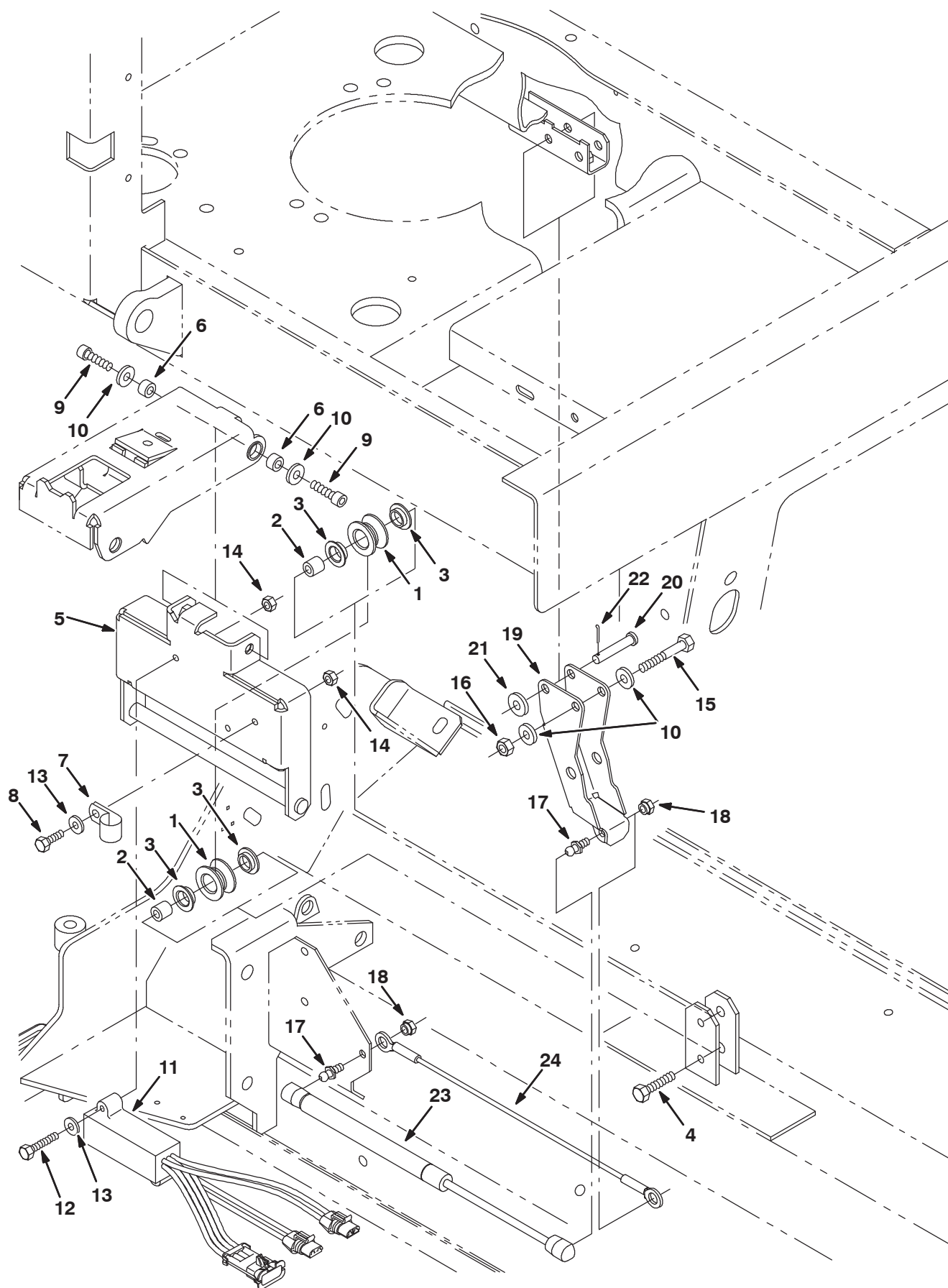
Fig. 33 - MaxPro 1200 (Cylindrical Brush) Edge Scrub Group
