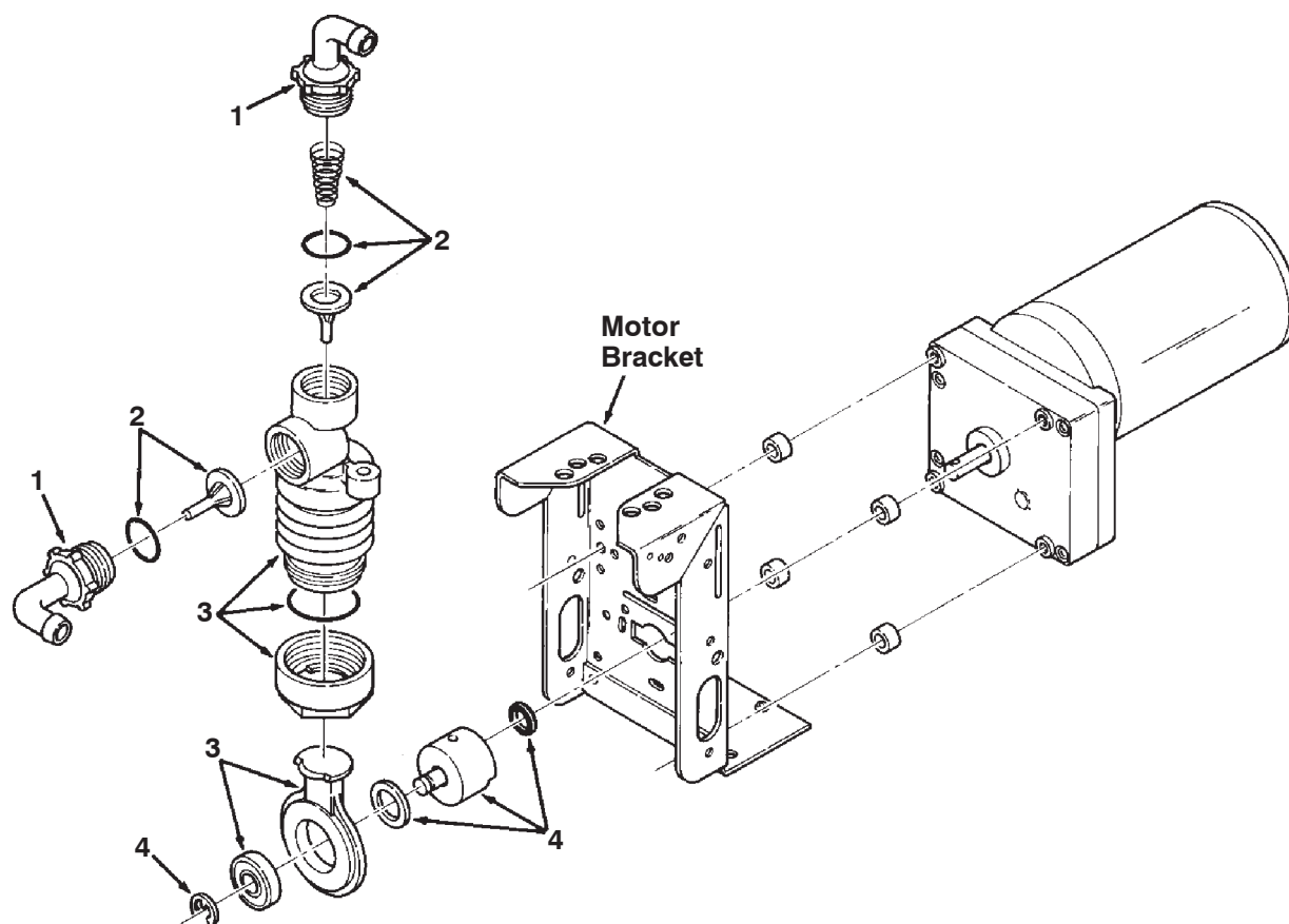
Fig. 12 - Metering Solution Pump Breakdown, 386364
