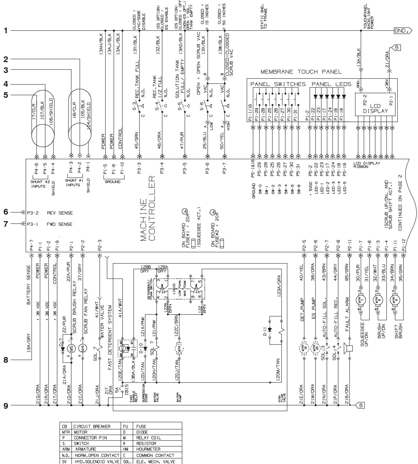
Fig. 63 - Electrical Schematic (1122- )
