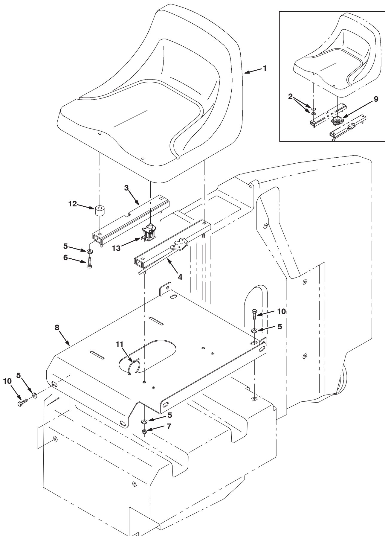
Fig. 8 - Seat Group
