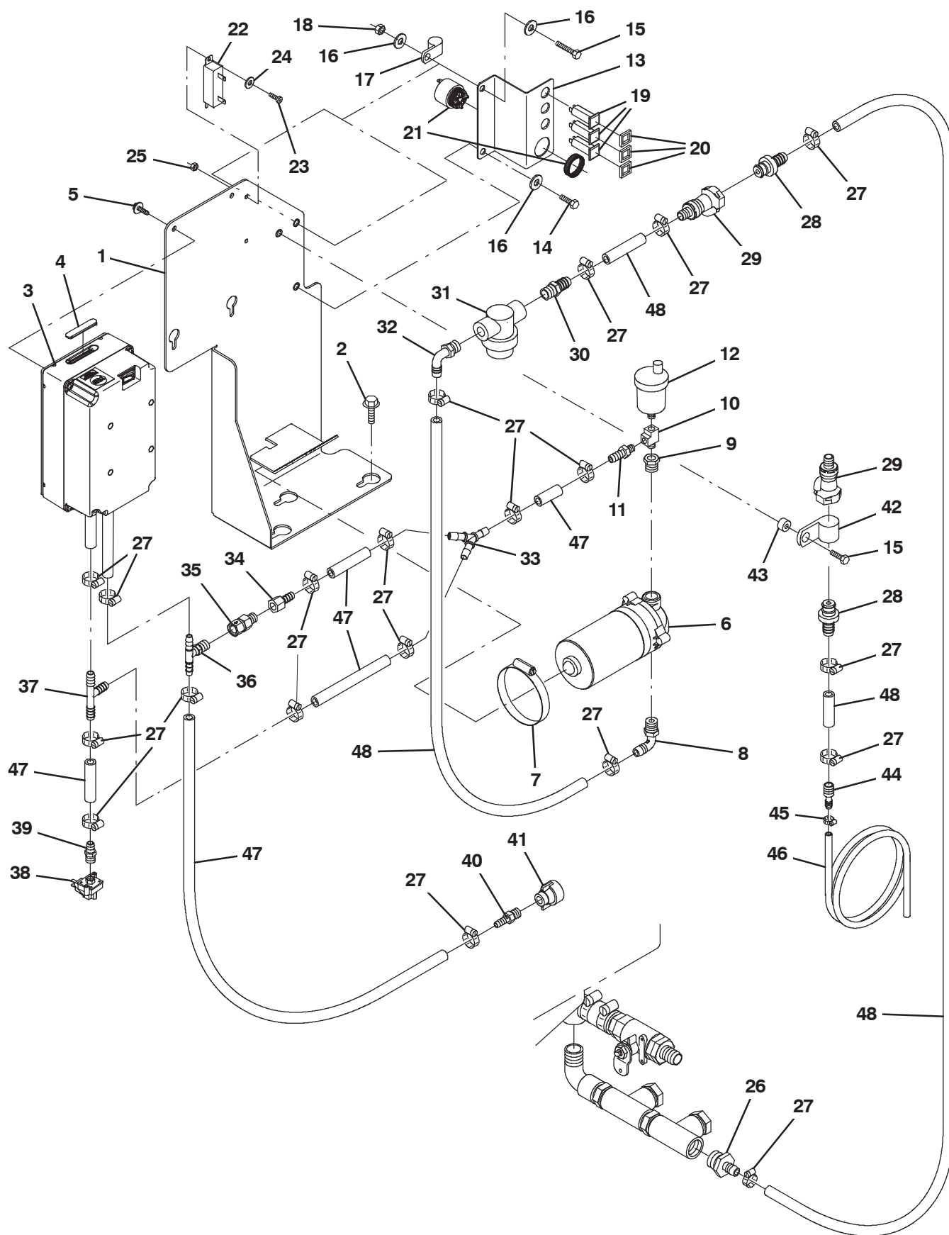
Fig. 37 - ec-H2O Solution Pump Group
