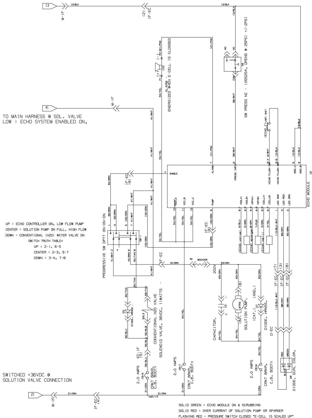
Fig. 63 - Electrical Schematic (1122- )
