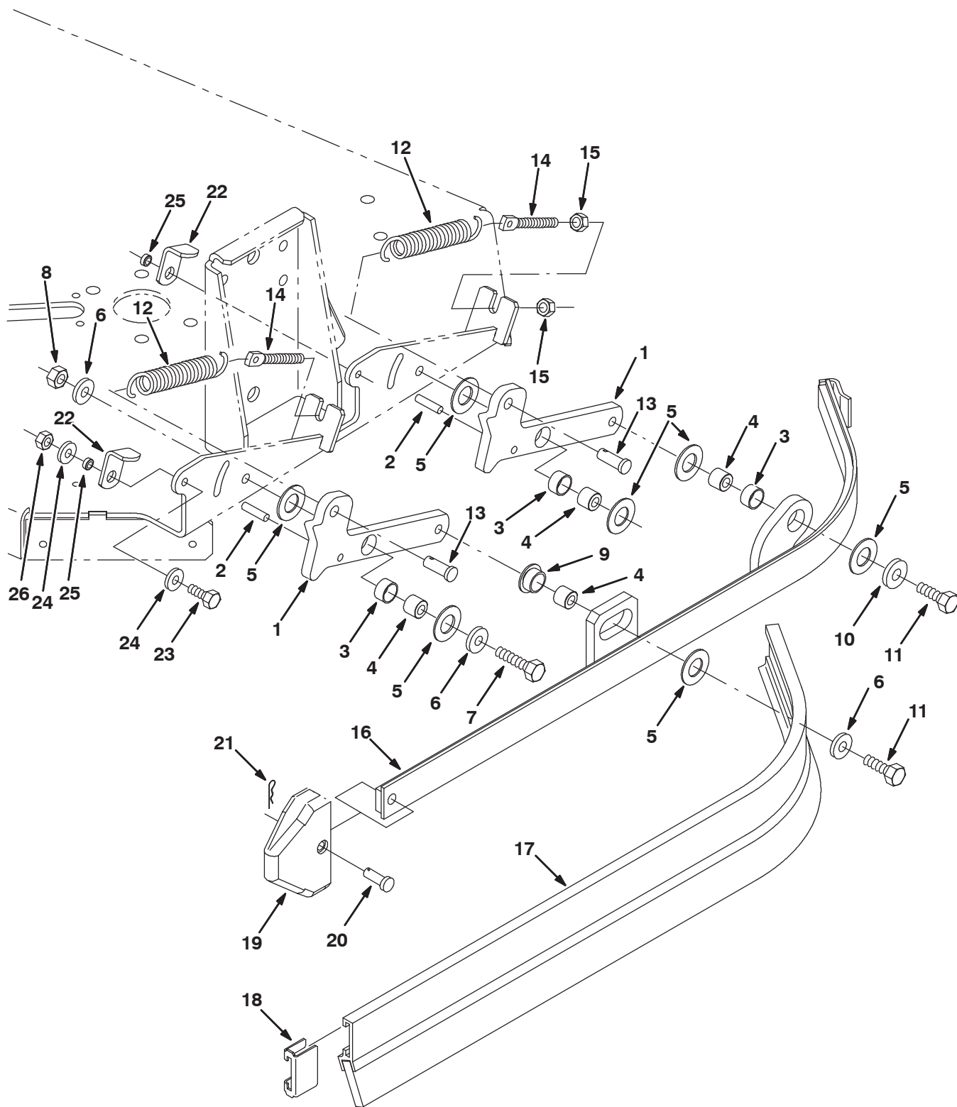
Fig. 34 - Max Pro 1000 (Disc—Brush) Left Side Squeegee Group
