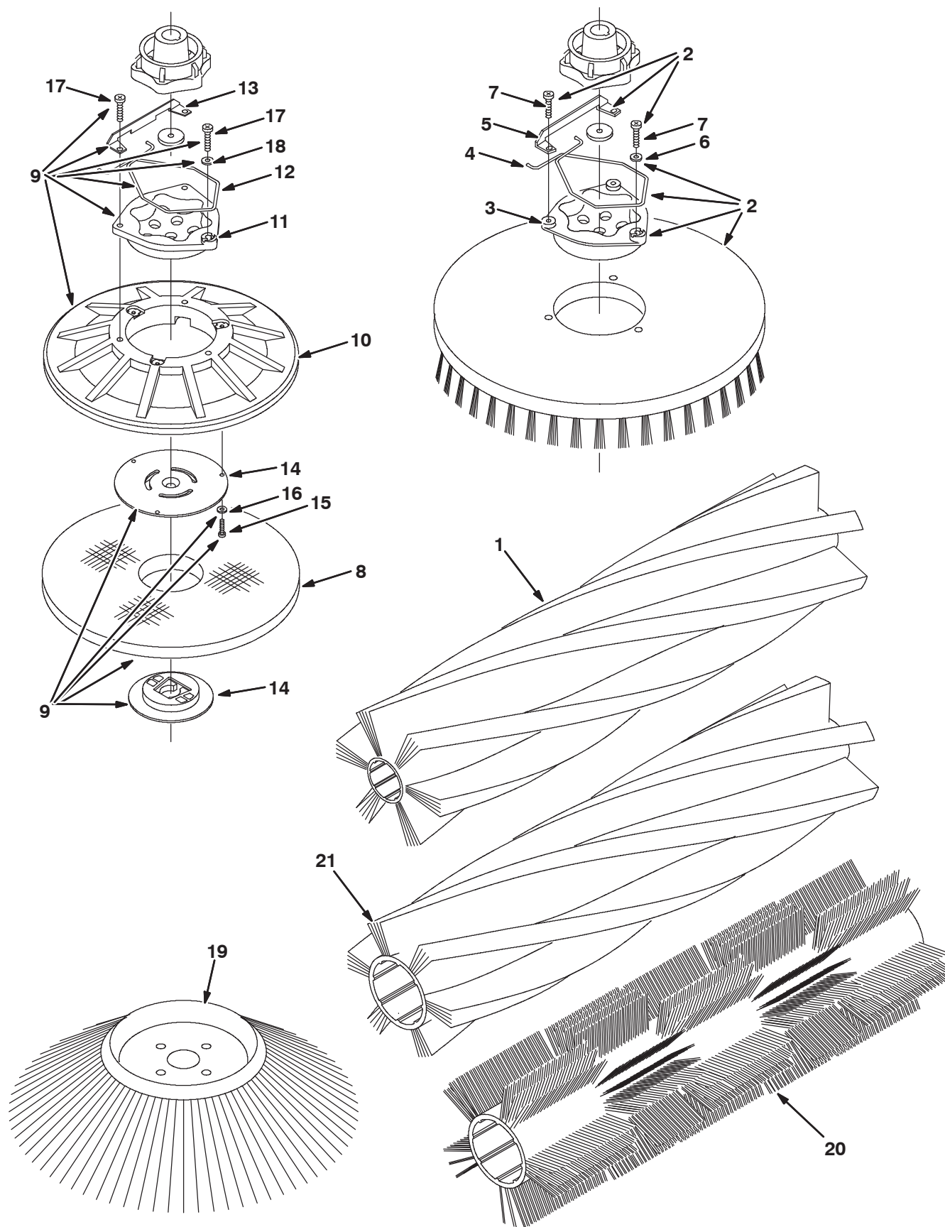
Fig. 1 - Replacement Brushes for Max Pro 1000
