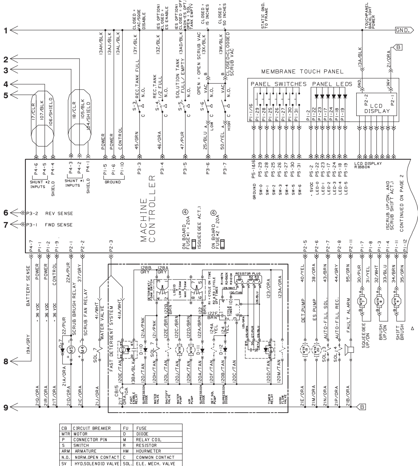
Fig. 62 - Electrical Schematic (0000-1121)
