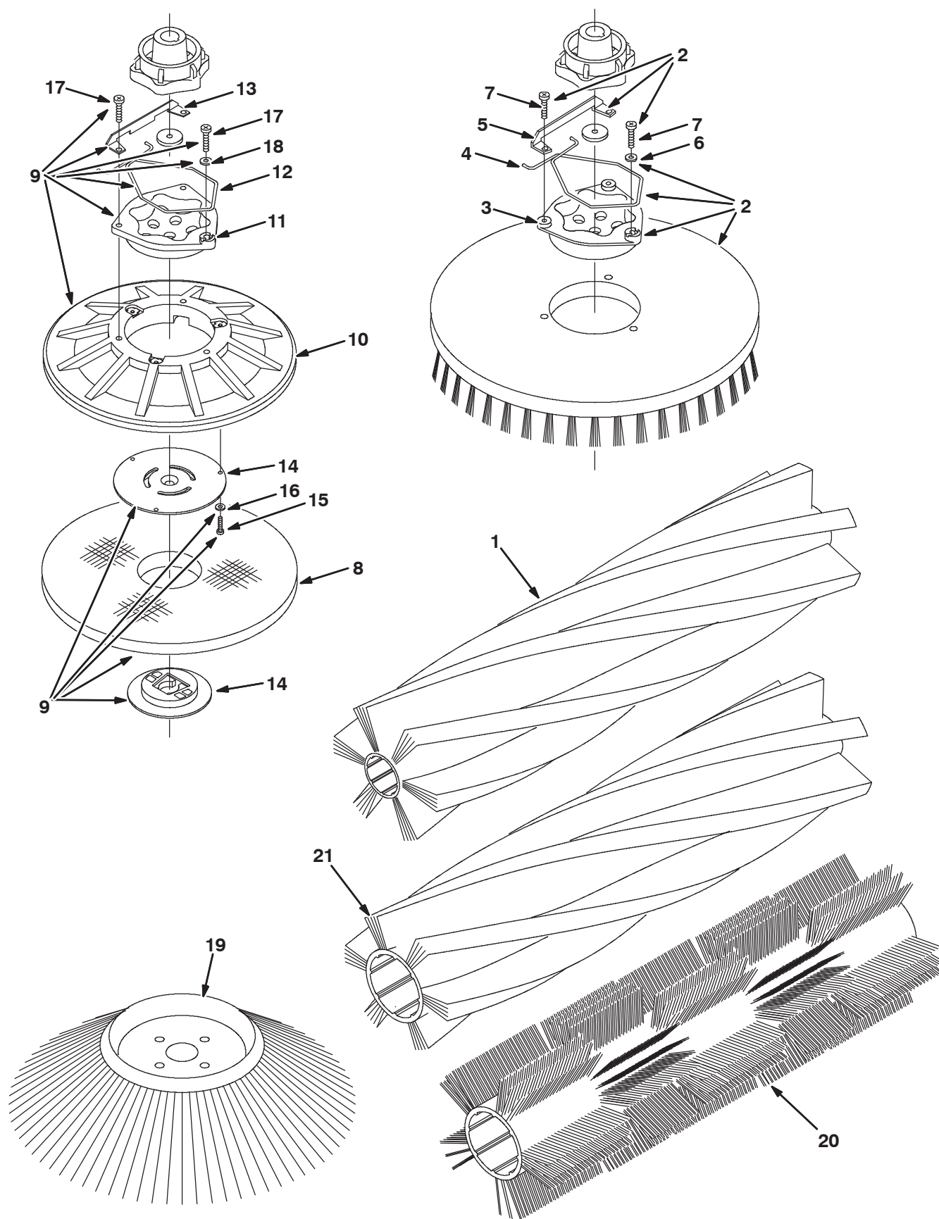
Fig. 2 - Replacement Brushes for Max Pro 1200
