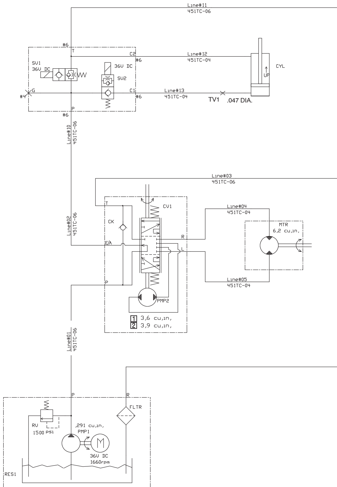
Fig. 52 - Hydraulic Schematic
