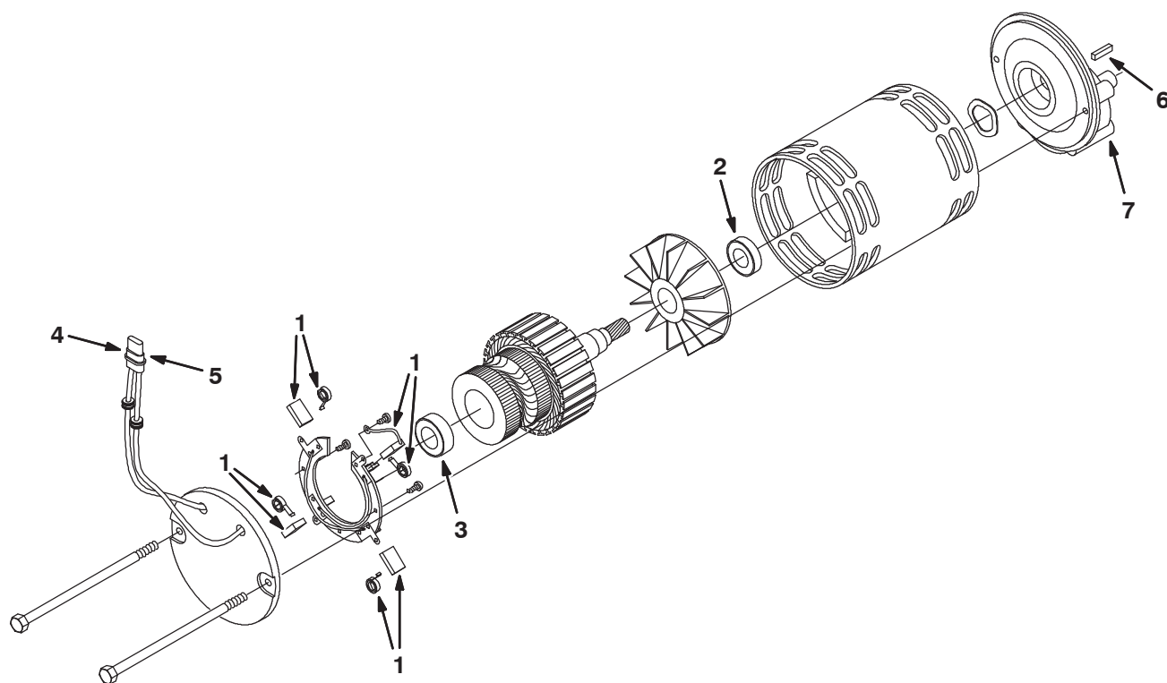
Fig. 10 - Electric Motor Breakdown, 386687
