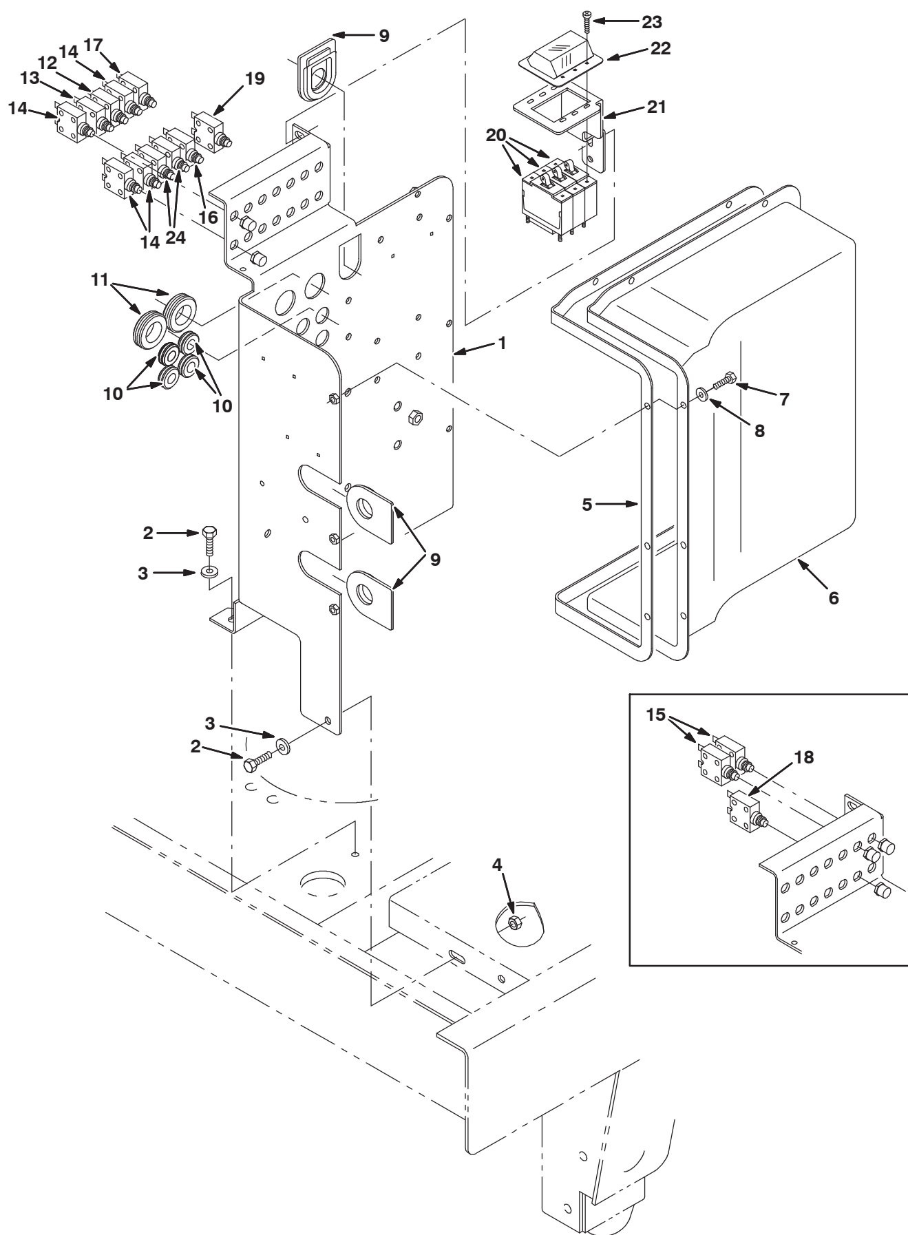
Fig. 54 - Control Box Circuit Breaker Group
