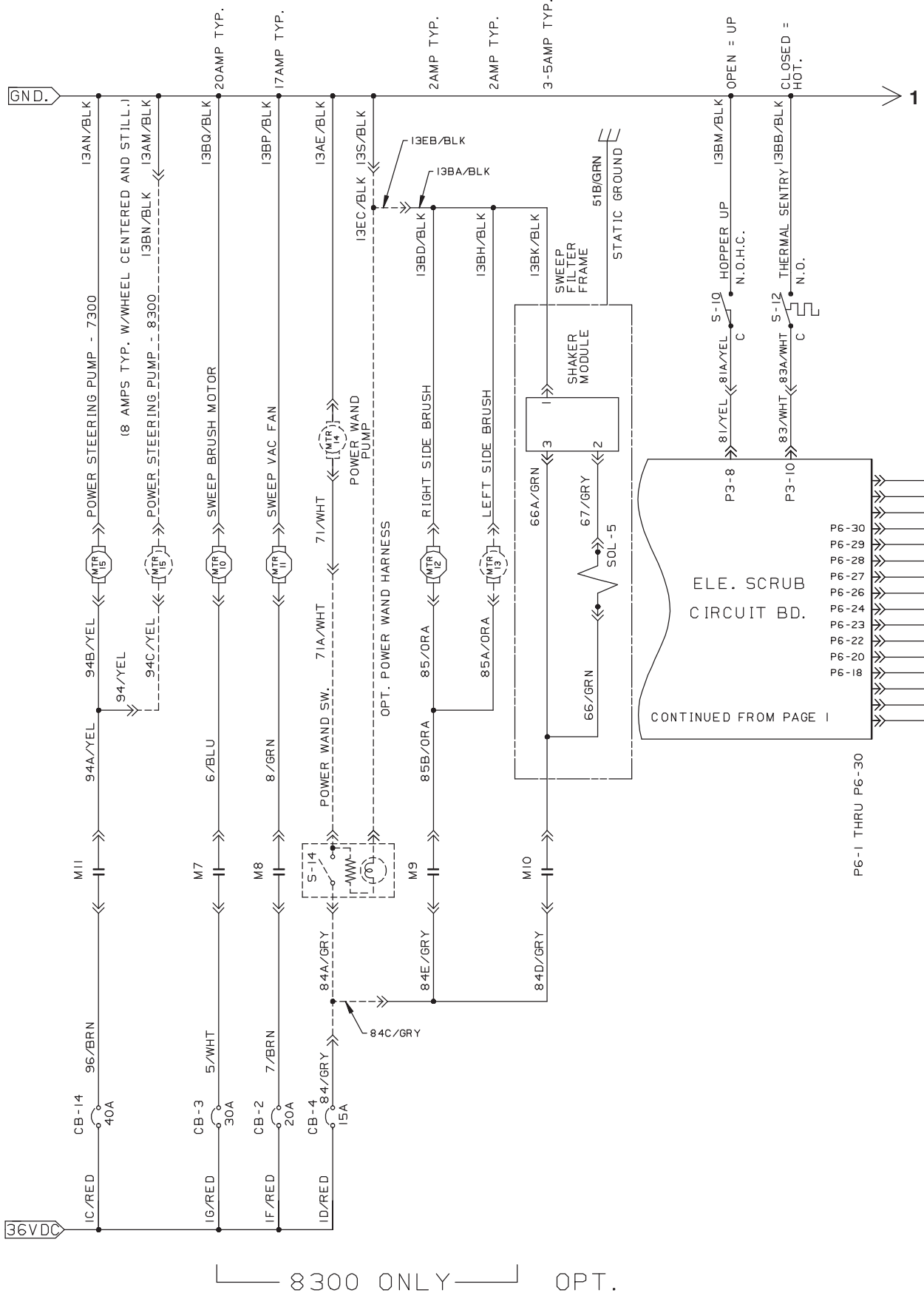
Fig. 62 - Electrical Schematic (0000-1121)
