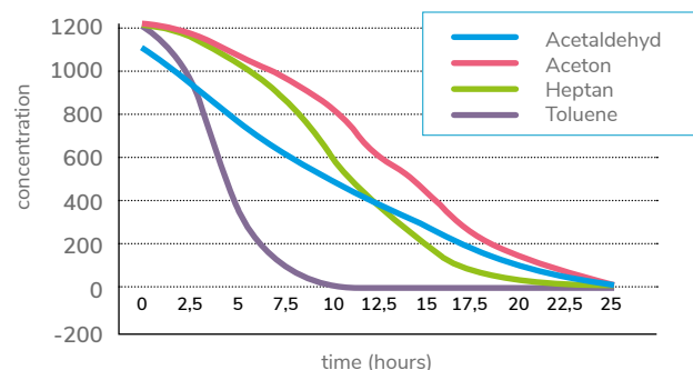
Reduction in VOCs on PURETI Clean&Fresh Treated Glass
